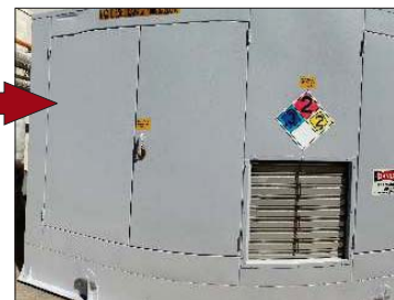
Electrical cabinet. Prepared by pressure washing then two coats of ENESEAL® CR.
